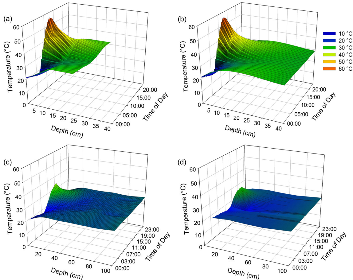
Fig. 4 Soil temperature profiles with increasing depth recorded in a, b the Negev desert highlands, Israel, and c, d the Kalahari desert, Namibia. Temperatures were recorded simultaneously for 24 h in August 2014 at a three locations in burrows of the scorpion Scorpio maurus at the entrance (2 cm deep), in the middle (11 cm deep), and at the bottom (22.5 cm deep) and b in an adjacent profile at 5-cm intervals from 0 to 40 cm deep in soil,
