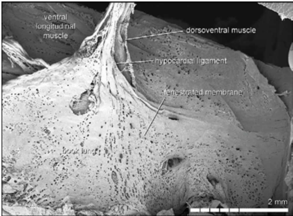
Fig. 7. Hadogenes sp., 1 ♂ (HUB): dorsolateral view of fenestrated membrane, covering sternite and book lung.
