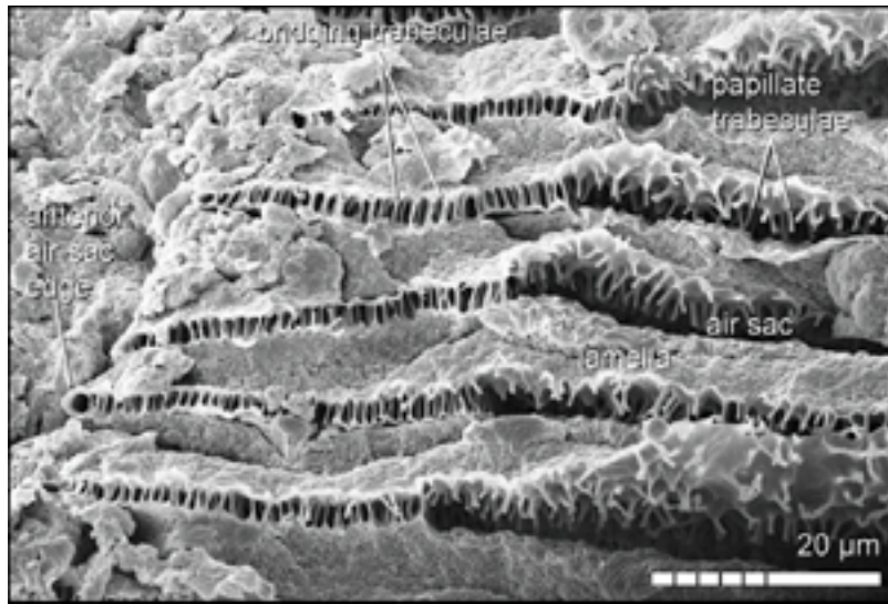
Fig. 12. Euscorpius carpathicus candiota Birula, 1903, 1 ♀ (HUB): lateral view of proximal parts of book lung (longitudinal section) showing lamellae and blind ends of air sacs.
