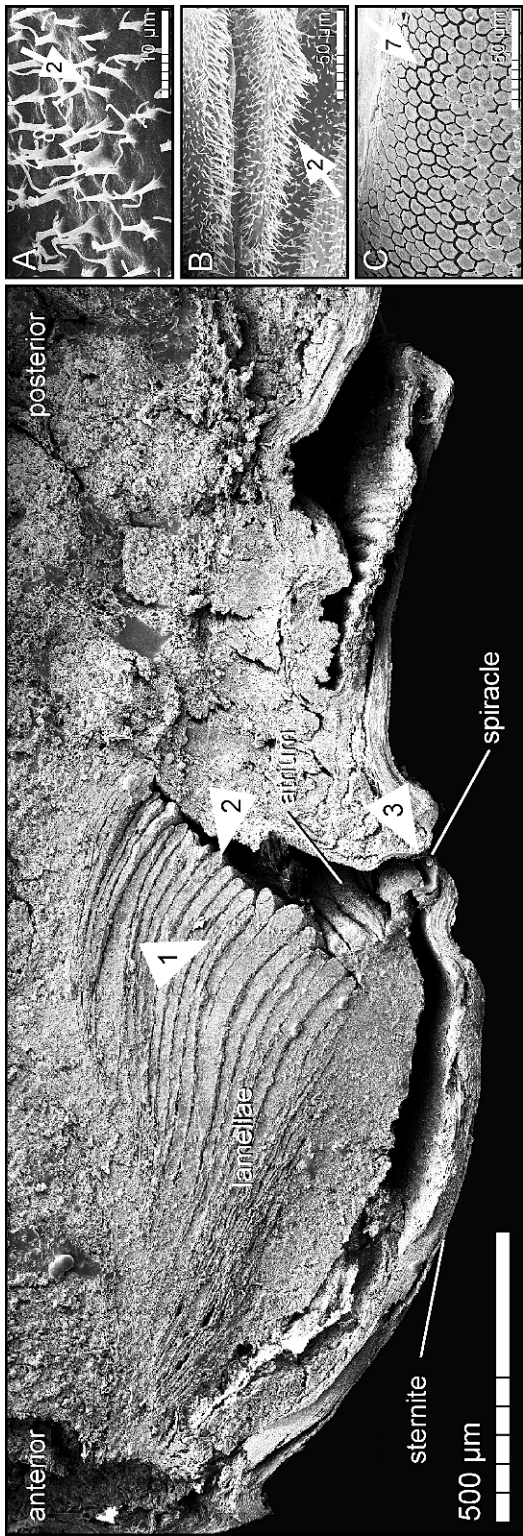
Fig. 4. Hottentotta jayakari (Pocock, 1895), 1 subad. ♀ (HUB): lateral view of longitudinal section through book lung, showing position of book lung morphology characters discussed in the atlas (arrowheads): lamellar surface (1); distal lamellar edge (2); posterior spiracle edge (3); (A–C) arrangement of characters in the plates, (A) lamellar surface, (B) lamellar edge, (C) posterior spiracle edge; arrowheads and arrows indicate characters and states.
