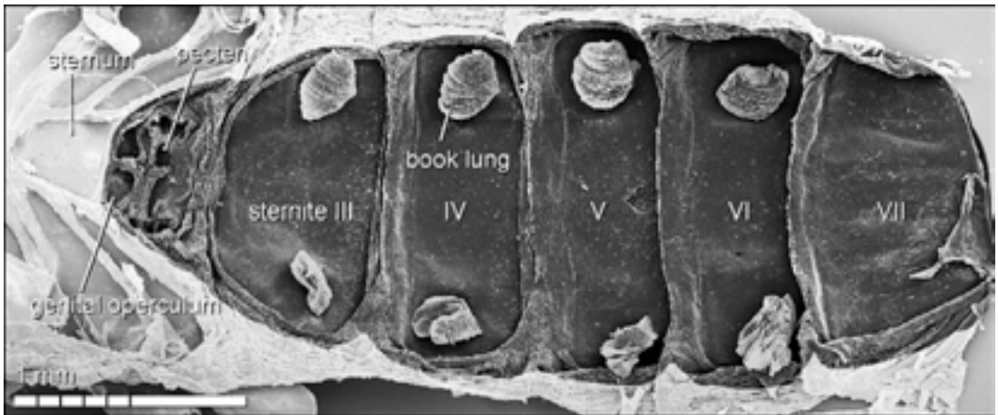
Fig. 2. Broteochoactas delicatus (Karsch, 1879), 1 juv. ♂ (AMNH), KOH-macerated cuticle: dorsal view of internal aspect of ventral mesosoma, showing location of book lungs.
