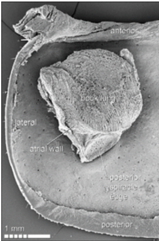
Fig. 9. Broteochoactas delicatus (Karsch, 1879), 1 ♂ (AMNH), KOH-macerated cuticle: dorsal view of lateral part of sternite, showing cuticular parts of book lung.
