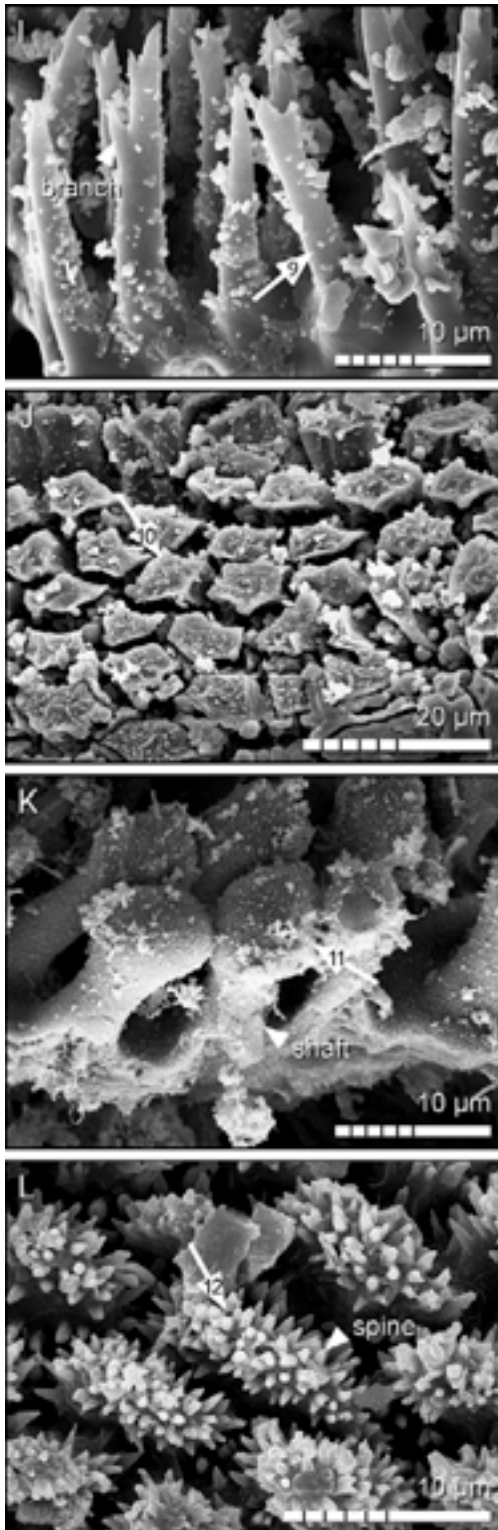
Fig. 17. Book lung, posterior spiracle edge (character 3): A. Karasbergia methueni Hewitt, 1913, 1 ♂ (AMNH [LP 1724]), state 1: hillocks (arrow); B. Orthochirus innesi Simon, 1910, 1 ♀ (MNHN RS 5440), state 2: subconical processes (arrow); C. Centromachetes pocockii (Kraepelin, 1894), 1 ♀ (ZMB 35145), state 3: hairlike processes (arrow); D. Urodacus yaschenkoi (Birula, 1903), 1 ♂ (AMNH [LP 1659]), state 4: flattened processes (arrow), pointed tips (arrowhead); E. Bothriurus coriaceus Pocock, 1893, 1 ♂ (ZMB 8322), state 5: scaly processes (arrow); F. Liocheles waigiensis (Gervais, 1843), 1 ♀ (MNHN RS 8350), state 6: chisel-like processes (arrow), distinct teeth (arrowhead); G. Scorpio maurus subsp., 1 ♀ (MNHN), state 7: hexagonal tiles (arrow), columellar shaft (arrowhead); H. Urophonius iheringii Pocock, 1893, 1 ♀ (AMNH [LP 3457]), state 8: treelike processes (arrow), branches (arrowhead); I. Centromachetes obscurus Mello-Leitão, 1932, 1 ♂ (AMNH [LP 2436]), state 9: subtree-like processes (arrow), short branches (arrowhead); J. Paruroctonus stahnkei (Gertsch and Soleglad, 1966), 1 ♂ (AMNH [LP 3566]), state 10: polygonal columns (arrow); K. Teuthraustes atramentarius Simon, 1878, 1 ♀ (MNHN RS 0784), state 11: clublike processes (arrow), slender shaft (arrowhead); L. Uroctonites huachuca (Gertsch and Soleglad, 1972), 1 ♀ (AMNH), state 12: spiked macelike processes (arrow), spikes (arrowheads); numbers in arrows refer to character states.
