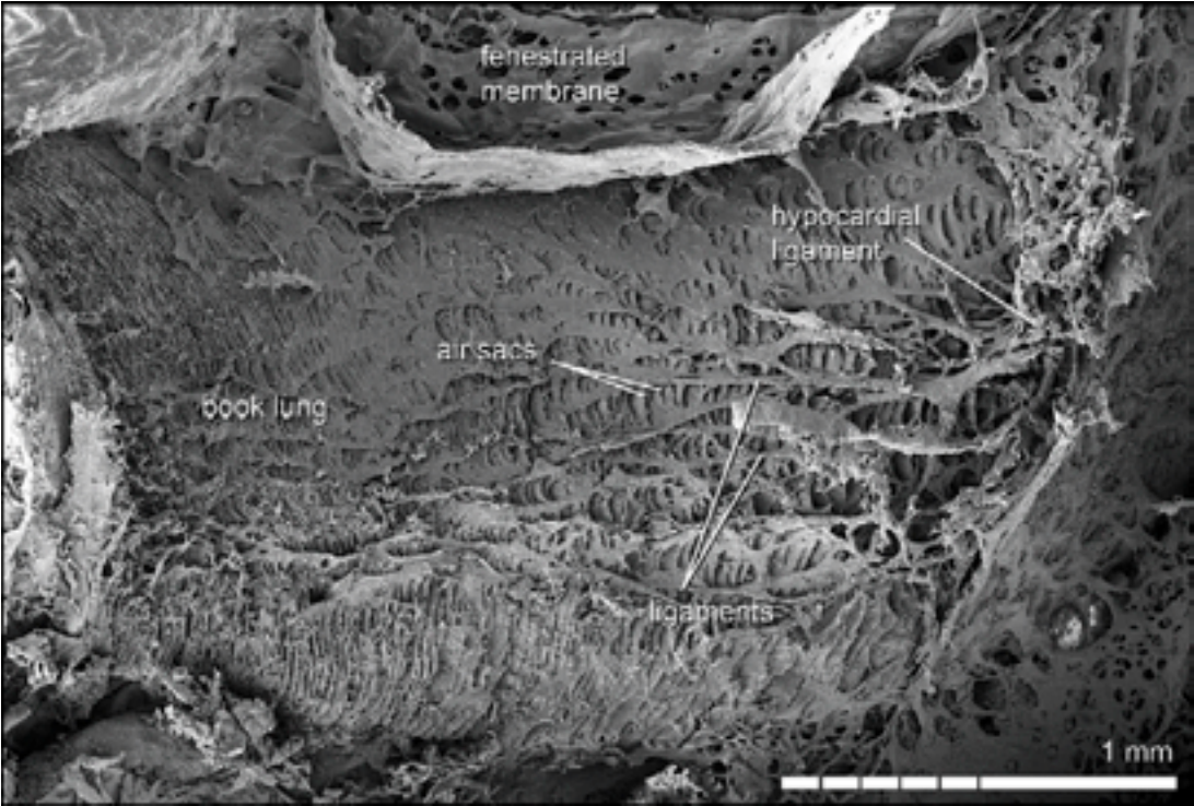
Fig. 6. Hadogenes sp., 1 ♂ (HUB): ventral view of book lung, with fenestrated membrane removed, showing ligaments holding air sacs.
