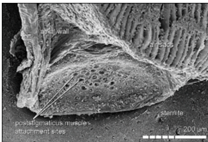
Fig. 14. Broteochoactas delicatus (Karsch, 1879), 1 ♂ (AMNH), KOH-macerated cuticle: dorsal view of attachment site of poststigmatic muscle on posterior edge of book lung spiracle. Posterior edge normally closes spiracle unless pulled open by contraction of poststigmatic muscle.
