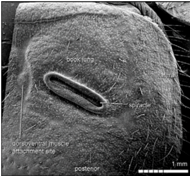
Fig. 3. Brotheas granulatus Simon, 1877, 1 ♂ (MNHN RS 8508): ventral view of dextral surface of sternite, showing position of spiracle, slanted with anterior margin (top) toward the midline (left).
