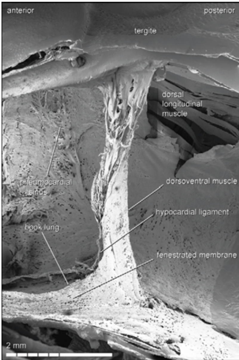
Fig. 8. Hadogenes sp., 1 ♂ (HUB): median lateral view of body cavity, with midgut removed.
